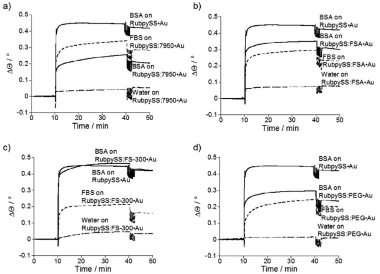
Figure 6. SPR sensorgrams of RubpySS and surfactant mixed monolayers. Surfactants used in each graph are Zonyl® 7950 (a), Zonyl® FSA (b), Zonyl® FS-300 (c) and PEG (d).
