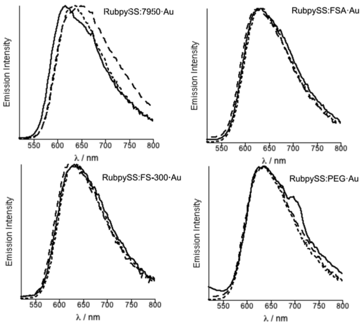
Figure 2. Steady state emission spectra of RubpySS without surfactant (short dash), co-coated with surfactant, before addition of BSA (solid) and after addition of BSA (long dash),. \lambda_{exc} = 465 nm, spectra corrected for instrument response. Spectral intensities are not to scale. BSA concentration is 16.5 \mu\text{M} . For simplicity of presentation Zonyl® 7950 is noted as 7950, Zonyl® FS-300 is noted as FS-300 and Zonyl® FSA as FSA.
