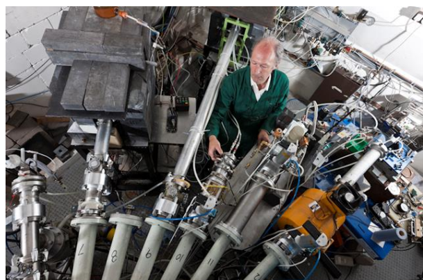
Figure 4: Beamlines emerging from the 12-way switching magnet: the lead enclosure houses one of the 81 Rb production targets.
