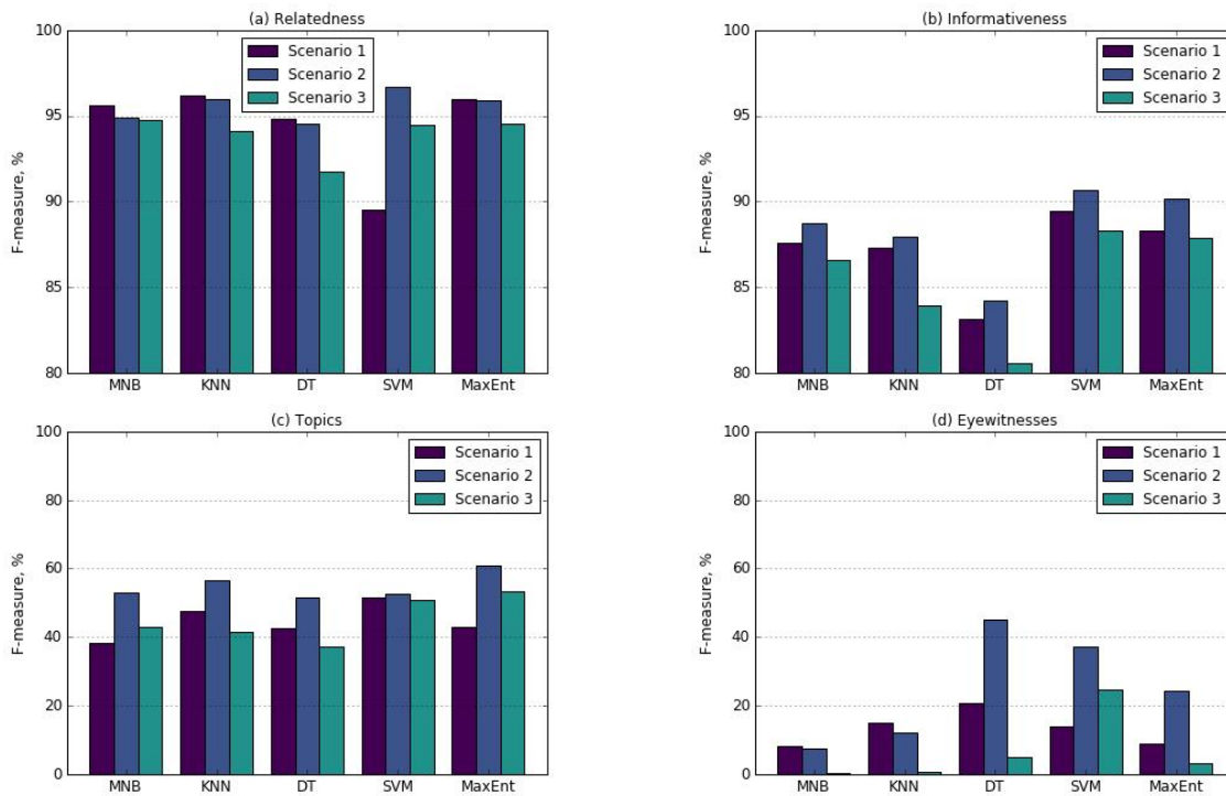
Figure 1. Comparison of F-measures achieved by the base learning methods on the Relatedness, Informativeness, Topics and Eyewitnesses tasks.
