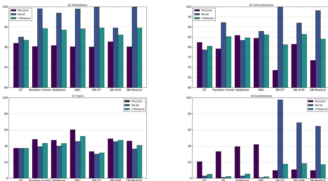
Figure 2. Performance of ensemble classifiers for the four evaluation tasks.
