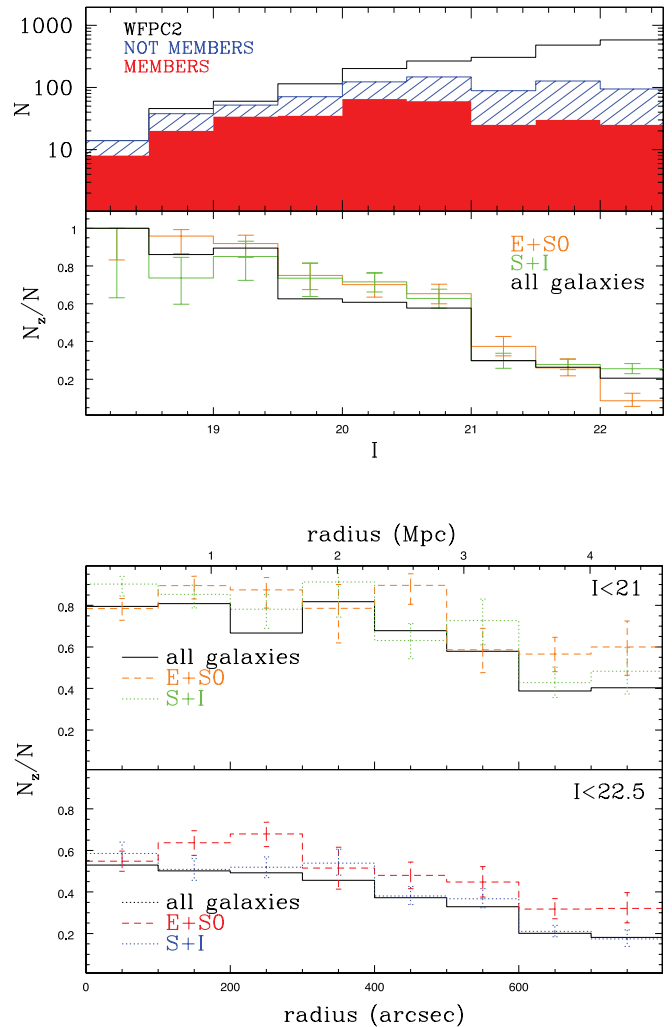
FIG. 3.—Top: Number counts as a function of I magnitude for all objects observed by WFPC2, with the number of cluster members and nonmembers marked (upper panel). For all objects with WFPC2 imaging, the lower panel displays the fraction with a measured redshift, as a function of I magnitude, and divided by morphology as indicated. Bottom: Fraction of objects with measured redshift, as in the top panel, but as a function of cluster radius, and to two separate magnitude limits, I < 21.1 (upper) and I < 22.5 (lower).
