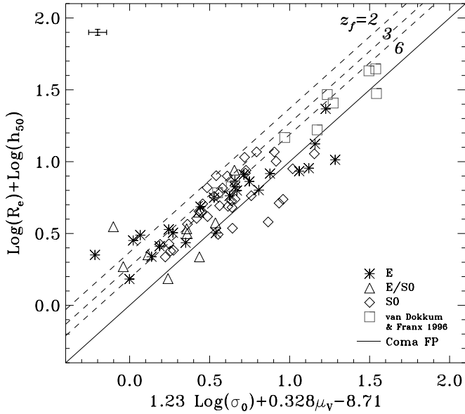
FIG. 5.—FP of Cl 0024, compared to Coma Cluster ( solid line ). Symbols represent different morphologies, as indicated. Dotted lines correspond to the expected shift in FP zero point from Coma to z \sim 0.4 , for SSP models with z_f = 2.0, 3.0, and 6.0 . [See the electronic edition of the Journal for a color version of this figure.]
