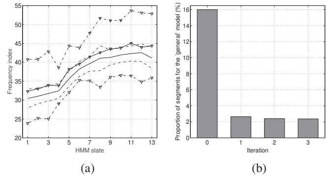
Fig. 6. The effect of the iterative label-reassignment training procedure on the HMM state output Gaussian PDF parameters (a) and on the number of segments assigned to the ‘general’ model (b).
