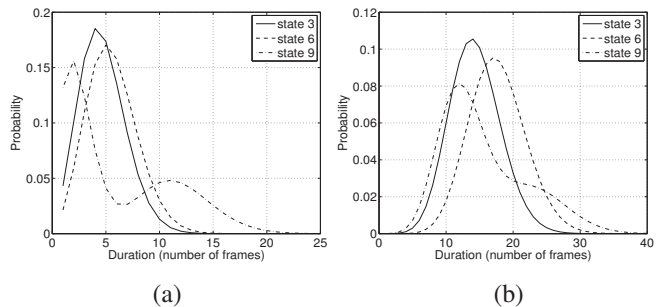
Fig. 5. Examples of the state duration models for several states of a bird element model when \tau = 0 (a) and \tau = 2 (b).
