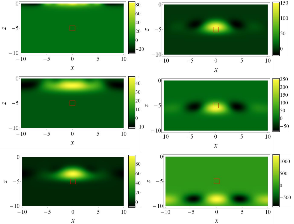
Figure 9 – Reconstruction of single square at z=-5m . Depth profiles for the left-hand column are centred at 0m , -2m and -4m . Depth profiles for the right-hand column are centred at -5m , -6m and -9m . The units are kg/m^3 .
