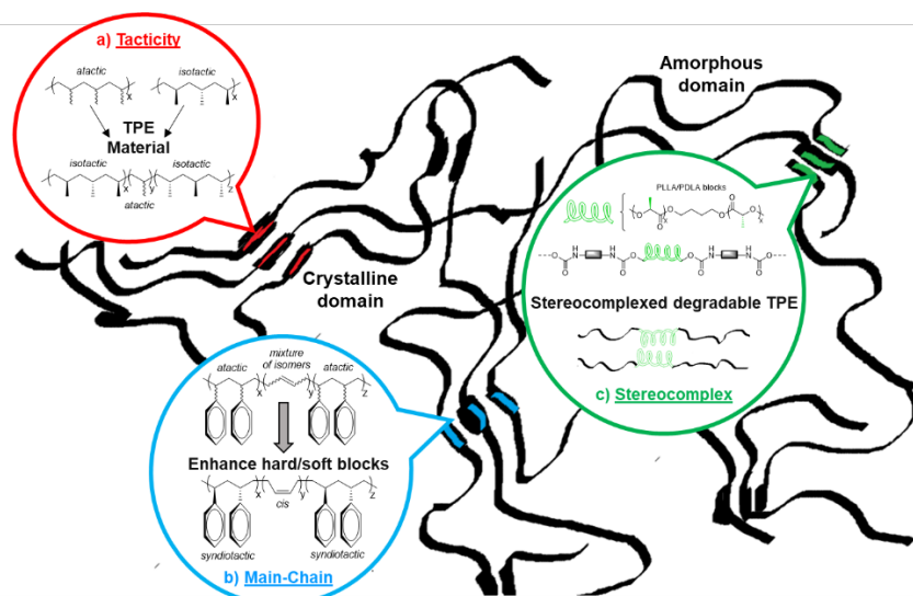
Figure 2. Examples of how stereochemistry can influence the mechanical properties of thermoplastic elastomers.
