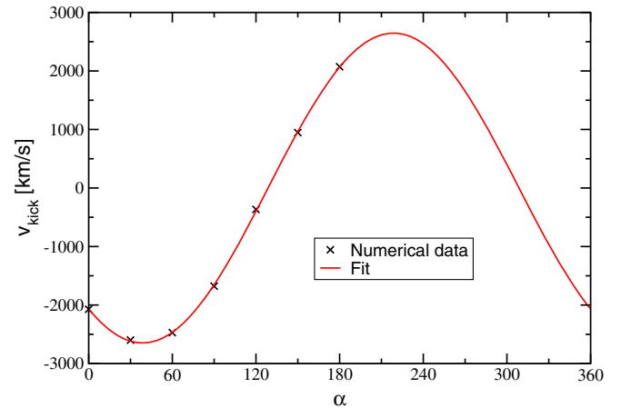
FIG. 3. The recoil velocity computed numerically from the GW signal for p = 0.075 is shown as \times symbols for different values of the spin orientation \alpha . The red curve represents the fit obtained from these data according to Eq. (3). Only data for \alpha < 180^\circ are needed to determine the fitting coefficients, due to the symmetry of the superkick configurations.
